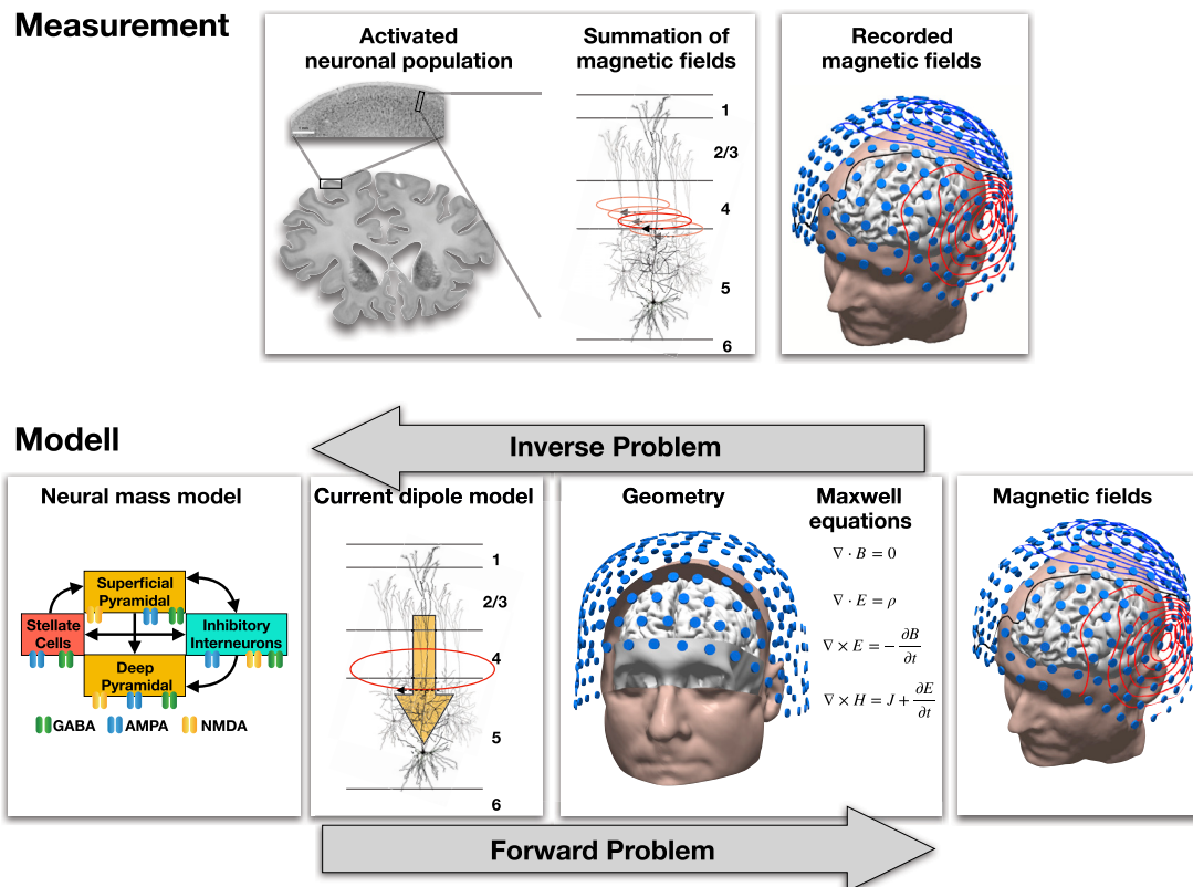
Figure 4. Forward and Inverse Problem
